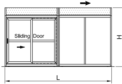
Side Elevation Closed
