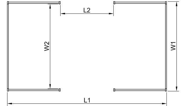
Plan View Section Opened
