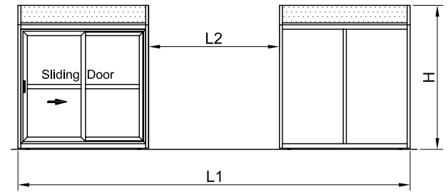
Side Elevation Opened
