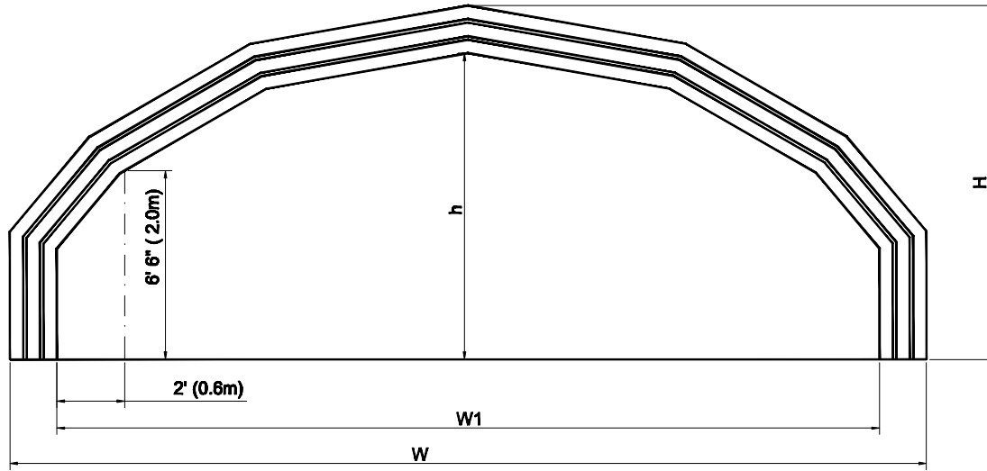
Section View
